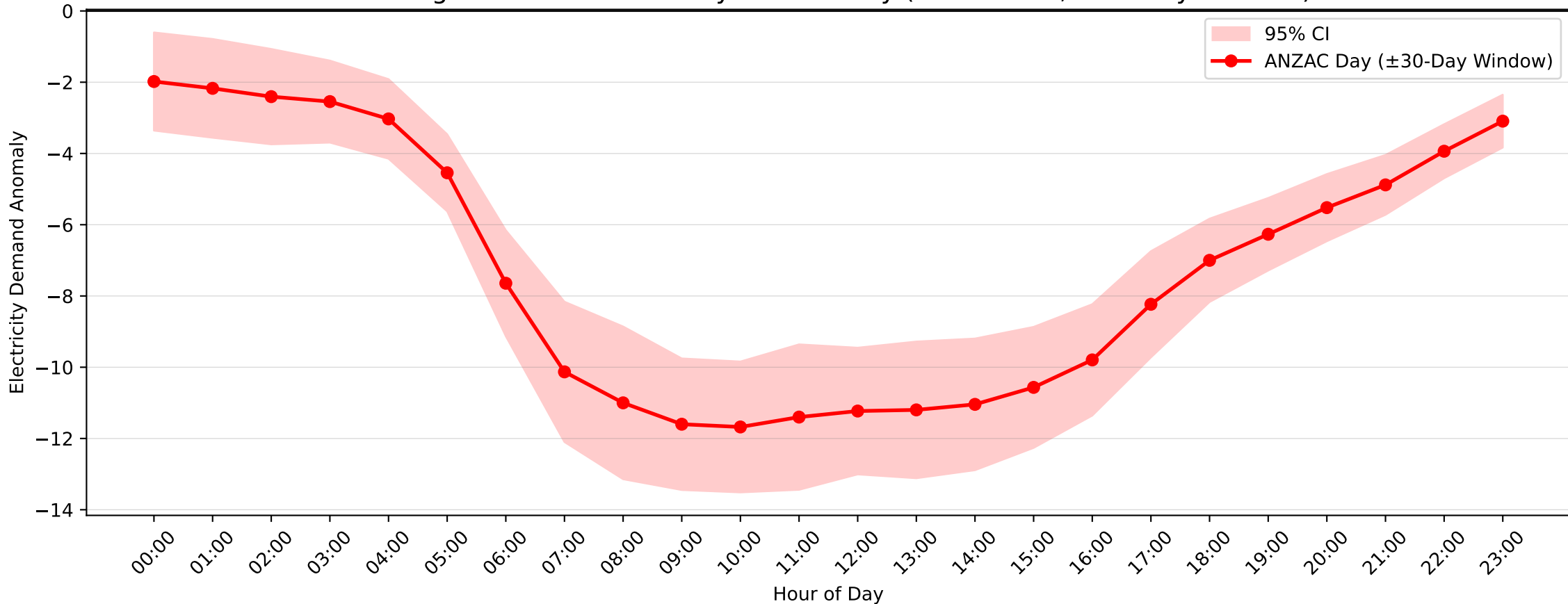
Flemington Demand Anomaly: ANZAC Day (2004–2017, \pm 30 -Day Window)
